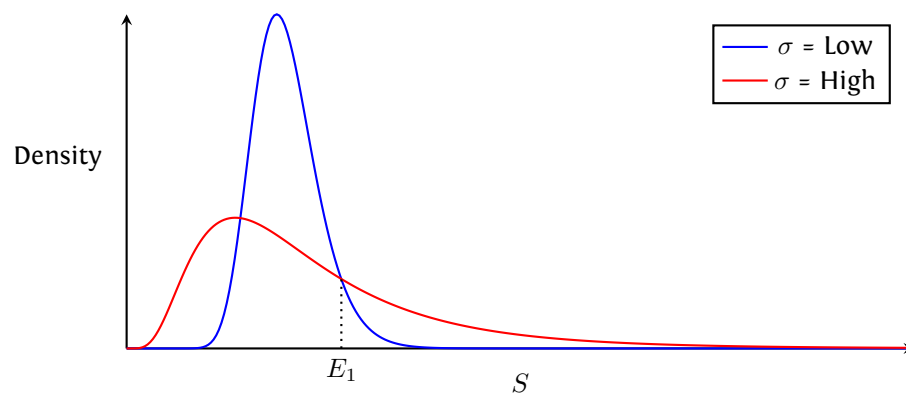
Figure 1: Lognormal distributions with low and high volatility
